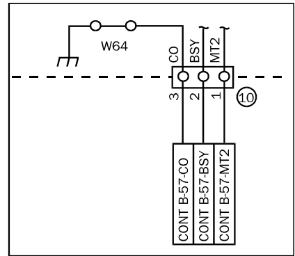
IF UNIT SCHEMATIC
